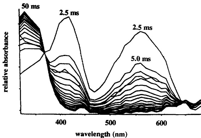
Figure 3. Time dependent UV-visible absorption spectra following stopped-flow admixture of flavinium salt (0.10 mM) and benzylamine (1.0 mM) in MeCN at 25°C. Each spectrum is recorded at 2.5 ms intervals following mixing over a 50 ms time interval.
