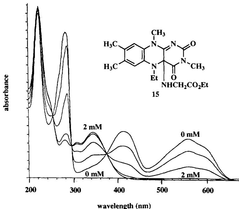
Figure 1. UV-visible spectrometric monitoring of the reaction of flavinium salt 1 (0.1 mM) with ethyl glycinate (0, 0.05, 1.0, 1.5 and 2.0 mM) in MeCN at 23°C to produce C4a-adduct 15 . Spectra are recorded immediately ( ca. 10s) after mixing.
