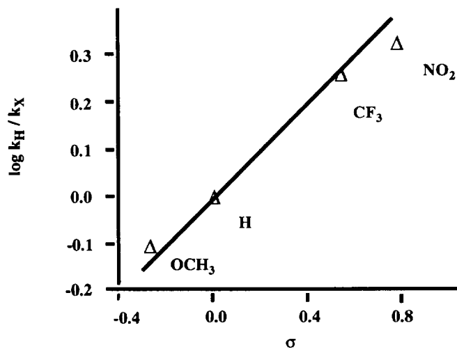
Figure 5. A linear free energy plot of the relative rates ( k_H/k_X ) of elimination of p -X-C 6 H 4 CH 2 NH 2 derived C4a-adducts 2 , 10-12 (from Table 2) vs. sigma.
