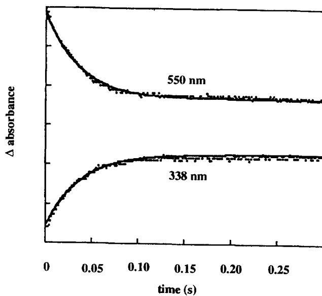
Figure 4. Plots of absorbance at 550 and 338 nm vs. time following mixing of flavinium salt 1 and benzylamine under the conditions described in Figure 3.
